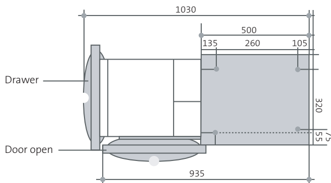
Outline drawing – horizontal section
