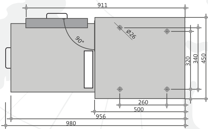
Outline drawing – horizontal section
